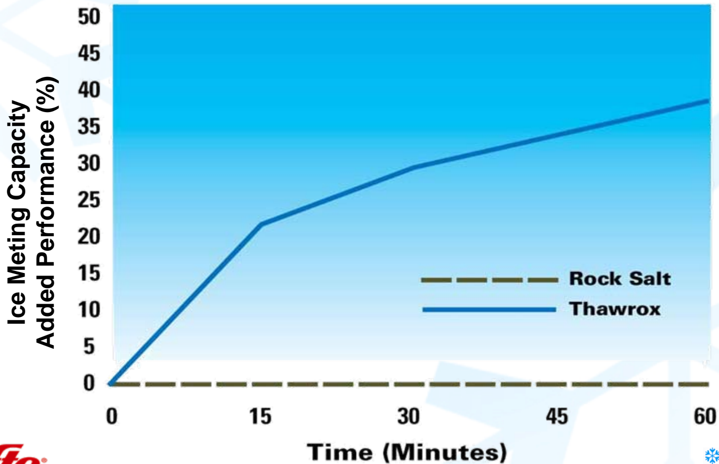
Melting Capacity of Thawrox at -15° C
